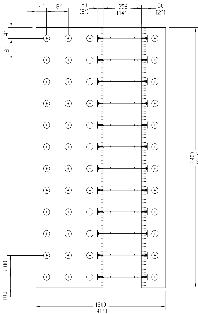
FRONT VIEW
