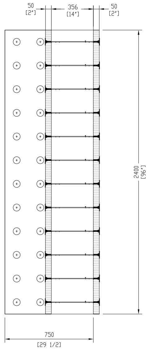
SIDE VIEW
