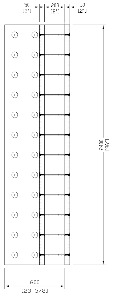
SIDE VIEW
